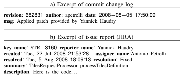
Figure 10. ReLink missed link – Unleveraged feature of links
