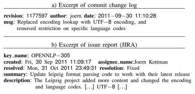
Figure 11. ReLink missed link – Excessive filtering
