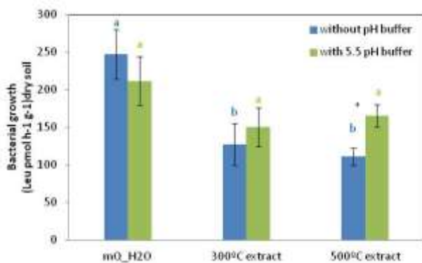
Figure 1. Mean values ( \pm SE, n=4 ) of bacterial growth estimated by leucine incorporation technique, under different incubation conditions (see section 2.3). Different letter with the same colour show significantly different mean values (Tukey's test, P < 0.05 ). "*" means significant differences in bacterial growth due to the addition of pH buffer (t-test, P < 0.05 ).
