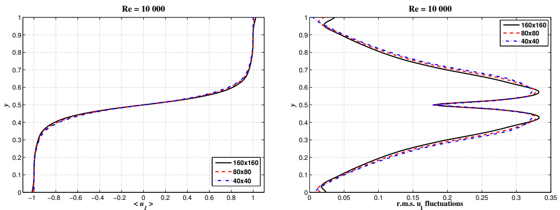
Figure 6: Example 5.2. Mean stream-wise velocity profiles (left) and r.m.s. stream-wise velocity fluctuations profiles (right) on different meshes.
