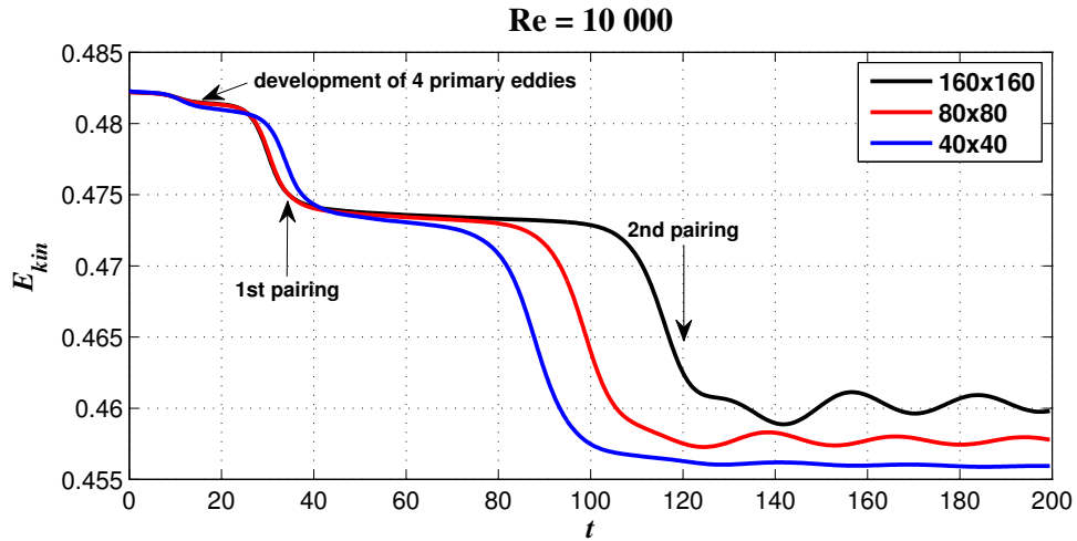
Figure 5: Example 5.2. Temporal evolution of the total kinetic energy on different meshes.
