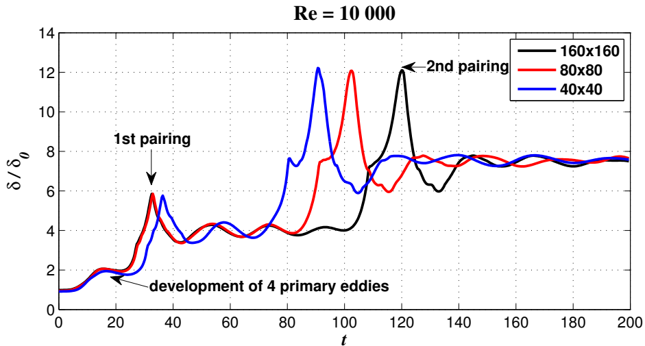
Figure 4: Example 5.2. Temporal evolution of the vorticity thickness on different meshes.
