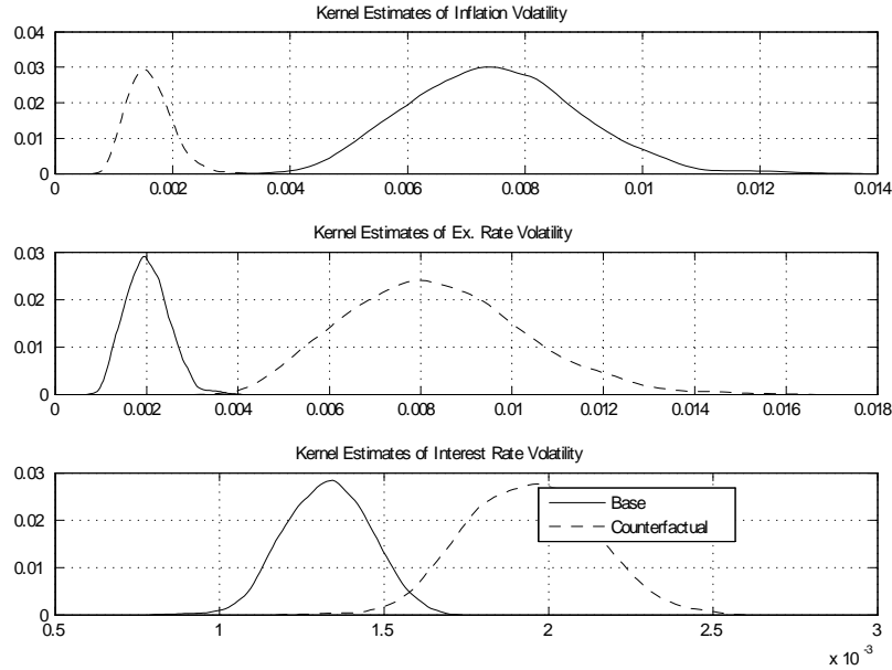
Figure 1: Inflation, Interest Rate and Exchange Rate Volatility under Base Policy and Counterfactual Taylor Rule
