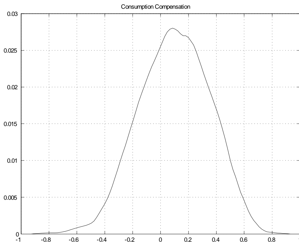
Figure 4: Consumption Compensation for Equalizing Welfare in the Two Regimes
