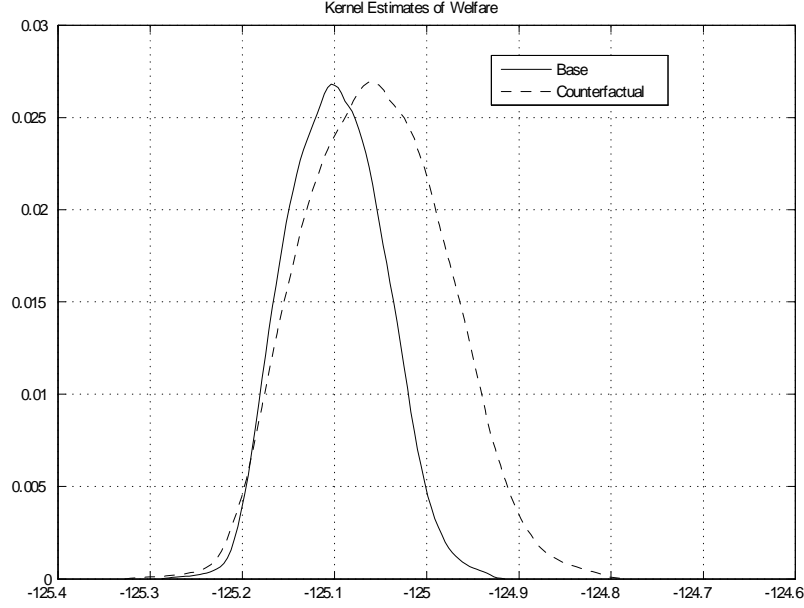
Figure 3: Welfare Distribution Under Base Policy and Counterfactual Taylor Rule
