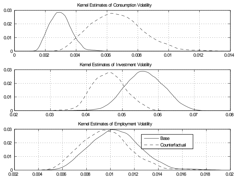
Figure 2: Consumption, Investment and Employment Volatility Under Base Policy and Counterfactual Taylor Rule
