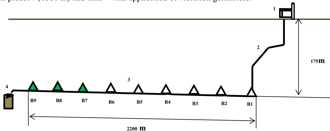
Fig.2. The diagram of vibration-pneumatic-gravity-flowing transportation of consolidating pulps from the stowing complex of Shokpak deposit to the shrink stoping of the deposit Kamyshovoye: 1 – stowing complex; 2 – vertical part of the pipeline; 3 – vibration generators; 4 – the stowing chamber of the block; B1-B9 – single-shaft vibration generators with electric motor drive
