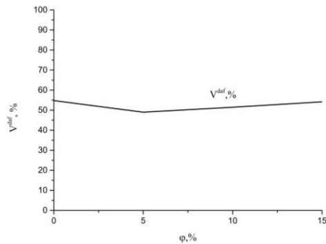
Fig. 5. Flour concentration effect on composite fuel volatiles yield in relation to mixture composition of coal and sawdust 50 % / 50 % ( \varphi – flour content)
