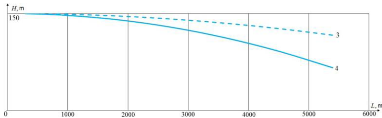
Fig. 2. The trajectory of the drops in winter: 3 – taking into account the process of evaporation; 4 – without taking into account the process of evaporation.
