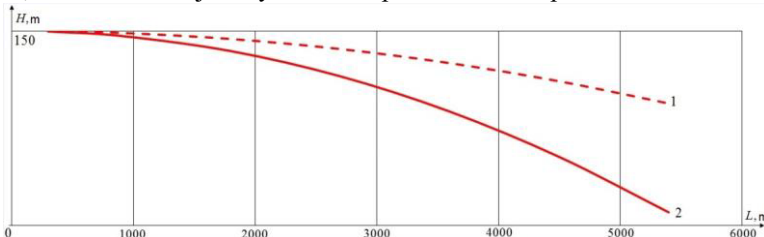
Fig. 1. The trajectory of the drops during the summer: 1 – taking into account the process of evaporation; 2 – without taking into account the process of evaporation.
