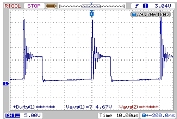
Fig. 6 The switching processes in the power switches of the CPS which is connected to the pipeline with improved insulation
