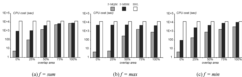
Fig. 46. CPU cost vs. overlap area ( P = LA , Q = TS , k = 4 ).
