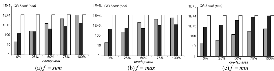
Fig. 47. CPU cost vs. overlap area ( P = TS , Q = LA , k = 4 ).
