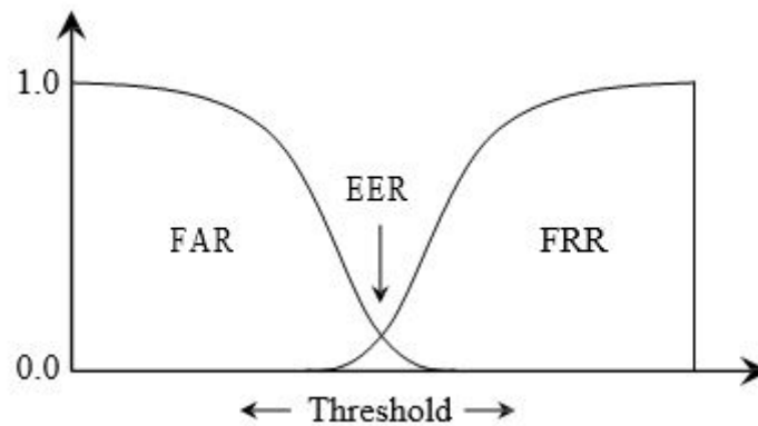
Figure 1.5: Values of the false acceptance rate (FAR) and the false rejection rate (FRR) for a varying threshold
