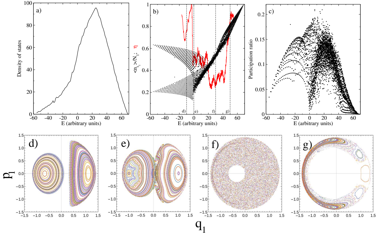
FIG. 11: Same as in Fig. ?? but for y = 0 , y' = 1 , and x = 1/2 . Panels d), e), f), and g) are Poincaré sections for energies E = -10 , E = 0 , E = 30 , and E = 50 .
