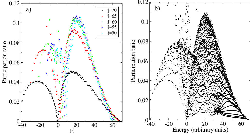
FIG. 5: Normalized participation ratio as a function of the excitation energy for the same Hamiltonian and parameters as in Fig. ???. a) For selected values of j , b) for all the states without distinction in j .
