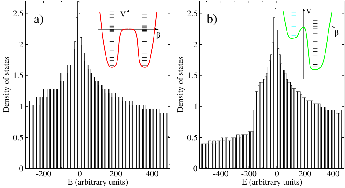
FIG. 2: Density of states for a one-fluid Lipkin Hamiltonian H = xn_t - \frac{1-x}{N}Q^{(y)} \cdot Q^{(y)} ( n_t and Q^{(y)} defined in (??) and (??) with x = 1/2 , y = 0 , and N = 1000 (panel (a)) and with x = 1/2 , y = 1/2 , and N = 1000 (panel (b)); the insets show schematically the corresponding potential energy surface in both cases.
