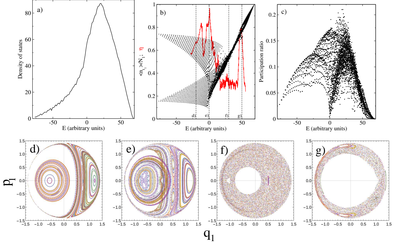
FIG. 12: Same as Fig. ?? but for y = 0 , y' = 3/2 , and x = 1/2 . Panels d), e), f), and g) are Poincaré sections for energies E = -20 , E = 0 , E = 30 , and E = 50 .
