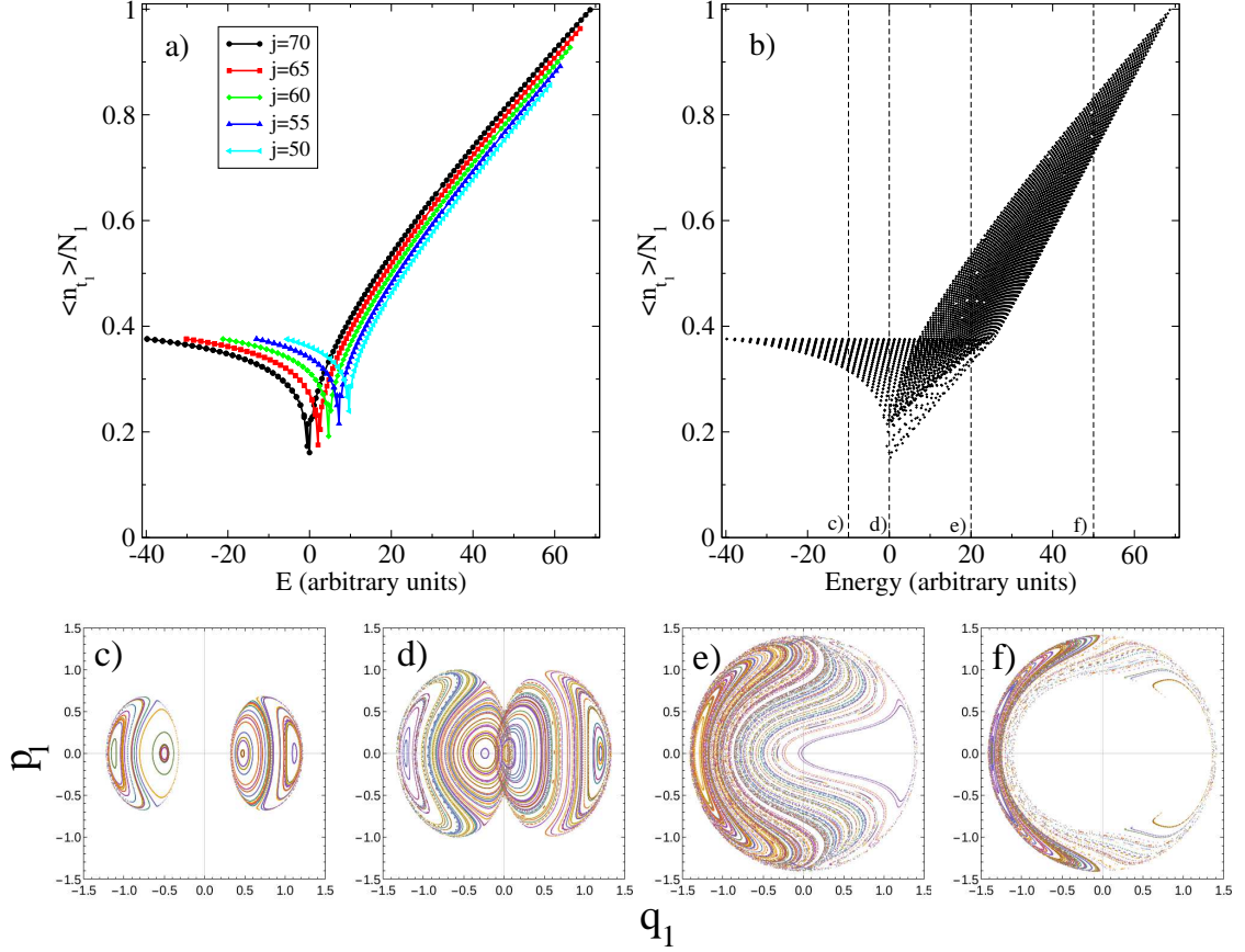
FIG. 4: Peres lattice for \frac{\langle n_{t_1} \rangle}{N_1} versus the excitation energy for the same Hamiltonian and parameters as Fig. ?? . a) For selected values of j , b) for all the states without distinction in j . Poincaré sections for energies E = -10 , E = 0 , E = 20 , and E = 50 , in panels c), d), e), and f), respectively (energies marked in panel (b)).
