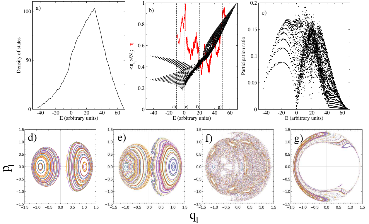
FIG. 10: Same as in Fig. ?? but for y = 0 , y' = 1/2 , and x = 1/2 . Panels d), e), f), and g) are Poincaré sections for energies E = -10 , E = 0 , E = 20 , and E = 50 .
