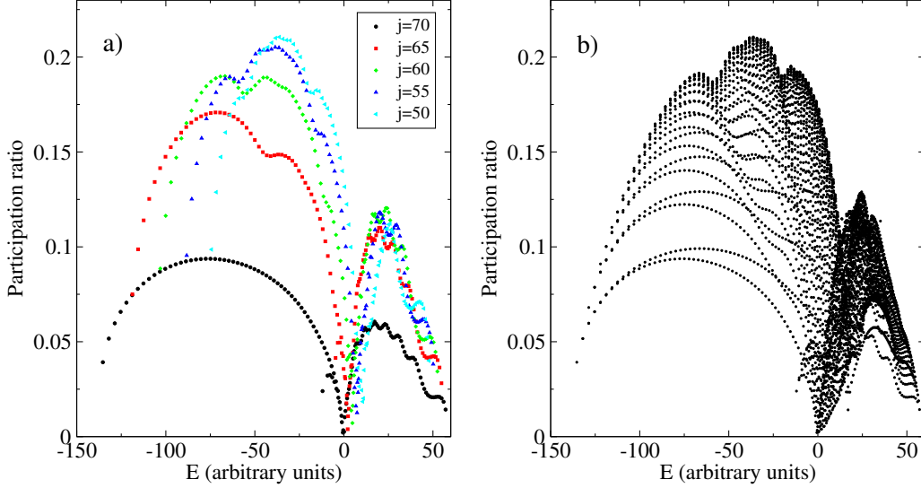
FIG. 8: Participation ratio as a function of the excitation energy for the same Hamiltonian and parameters as in Fig. ?? . a) For selected j -values, b) for all the states without distinction in j .
