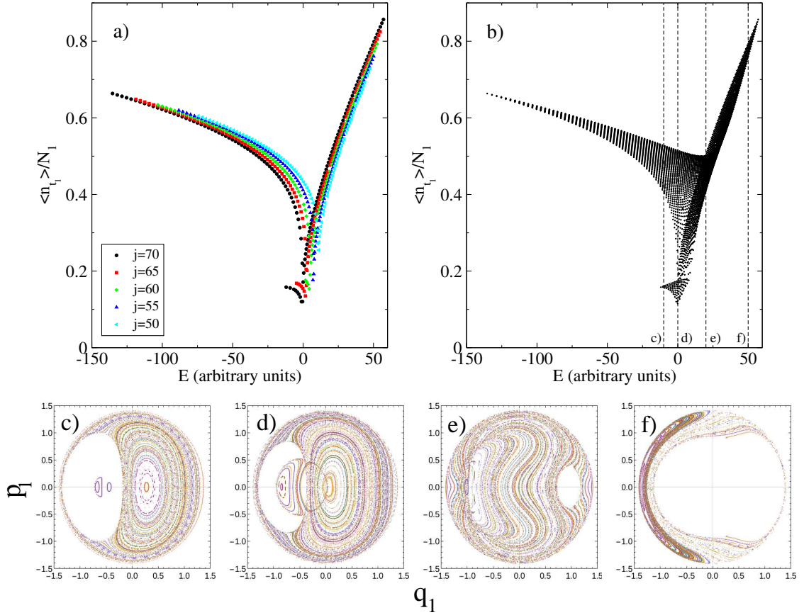
FIG. 7: Peres lattice for \frac{\langle n_{l_1} \rangle}{N_1} versus the excitation energy for the same Hamiltonian and parameters than in Fig. ???. a) For selected values of j , b) for all the states without distinction in j . Poincaré sections for energies E = -10 , E = 0 , E = 20 , and E = 50 , in panels c), d), e), and f), respectively (energies marked in panel (b)).
