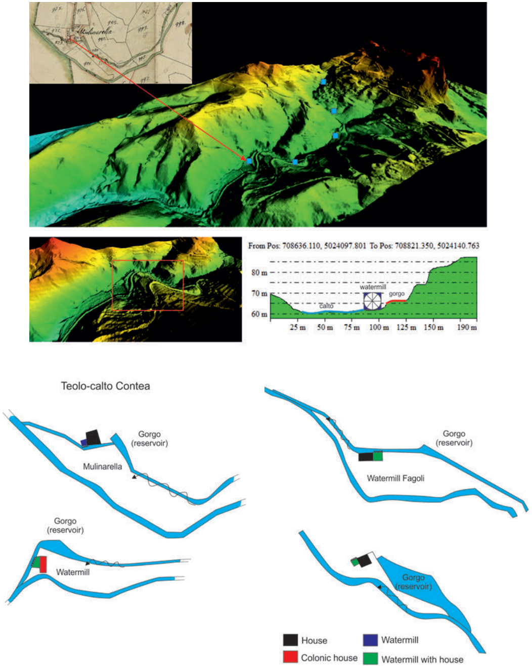
Fig. 10. Watermills on the Calto della Contea showing the typical structure of water mill factories in the Euganean Hills.
