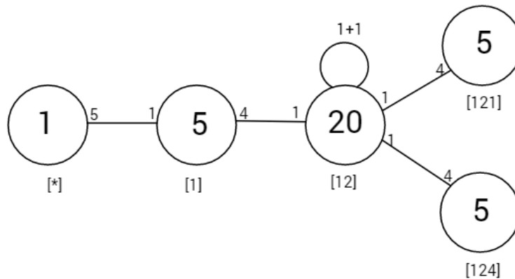
Figure 6.1: Cayley diagram of S_6 over (5 : 4)
