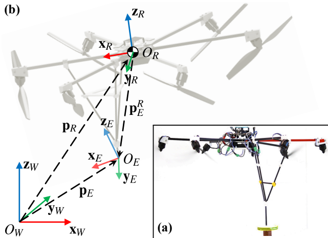
Fig. 1: a) The Tilt-Hex (NCFTP platform in-house developed at LAAS-CNRS) with the rigidly attached end-effector in contact with a force torque sensor used as ground truth. Notice how the interaction takes place far away and off-centered from the vehicle CoM. b) Schematic view of important frames and vectors.
