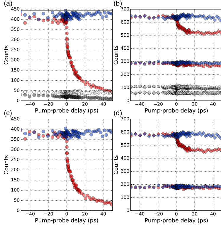
FIG. S4: Raw data and background subtraction. (a) & (b) Summed up raw data for a set of delay scans for a particular pump fluence ( 1 \text{ mJ/cm}^2 ). The pumped signal is denoted with red and the unpumped signal with blue symbols. The respective halo backgrounds are the dark grey symbols (pumped) and light grey symbols (unpumped). Plot (a) exhibits the raw data for the antiferromagnetic case and (b) for the ferromagnetic case. In the latter the diamonds denote positive and the pentagons negative magnetization direction. (c) & (d) Respective delay scans after background subtraction.
