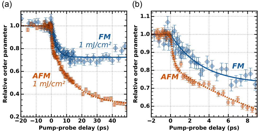
FIG. 2: (a) Pump-probe delay scans in the FM (blue) and AFM (orange) phase for an absorbed laser fluence of 1 \text{ mJ/cm}^2 . The symbols denote the normalized magnetic order parameter; the lines denote exponential fits to the data. (b) First 9 ps of the delay traces on an enlarged scale.
