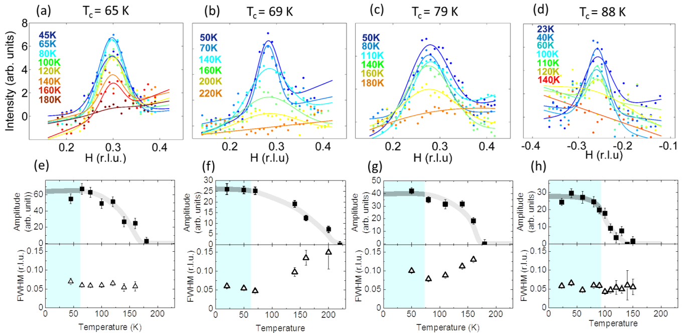
FIG. 4. (color online) (a-d) Temperature dependence of the background-subtracted CDW peak for four Hg1201 samples observed by RXS. The peak intensity decreases above T_c and saturates at the characteristic doping-dependent temperature T_{CDW} . In order to obtain the most accurate temperature dependence of the CDW peak parameters, high-temperature data were subtracted from the low-temperature scans (i.e., data at 200 K, 240 K, 200 K and 155 K were selected as reference background for the samples with T_c = 65 K, 69 K, 79 K and 88 K, respectively). The solid lines are the result of subsequent Gaussian-function fits. (e-h) Temperature dependence of the peak amplitude and width (FWHM). Blue areas indicate the superconducting state for each sample. The thick gray lines are guides to the eye.
