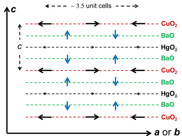
FIG. 9. (color online) Illustration of the average atomic displacements proposed for the CDW order in Hg1201. The red, green and black dashed lines correspond to the \text{CuO}_2 , BaO and \text{HgO}_8 layers, respectively. Black (blue) arrows represent the longitudinal (transverse) atomic displacements. Small and large displacements are indicated by the length of the arrows (not to scale). See the text for further details.
