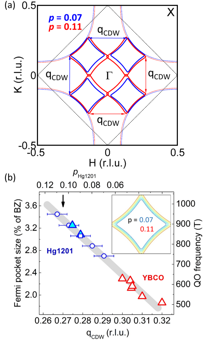
FIG. 7. (color online) (a) Noninteracting tight-binding FS of Hg1201 at p = 0.07 (light blue) and p = 0.11 (light red) with hopping parameters from Ref. 72 . Thick lines: reconstructed electron pocket; double-arrows: q_{CDW} (see main text). (b) Pocket size, as a fraction of the Brillouin zone, and associated quantum-oscillation frequency ( F ) for Hg1201 and YBCO as a function of q_{CDW} . Blue square (Hg1201) 20,45 and red triangles (YBCO) 61 represent the doping levels for which both q_{CDW} and F have been determined experimentally. F is related to the Fermi pocket size S via the Onsager relation, F = \hbar S/2\pi e . Blue circles: pocket size estimated from tight-binding calculation, with q_{CDW} obtained from the linear fit in Fig. 6(b). Horizontal error bars: experimental uncertainty in q_{CDW} . Blue triangles: recent high-precision experimental result for F . 21 Inset: doping dependence of the electron pocket in the reduced Brillouin zone (increments: \Delta p = 0.01 ). Predicted Lifshitz-type change in FS topology at p \approx 0.105 (black arrow) due to overlap of reconstructed pockets (see result for p \approx 0.11 in panel (a)).
