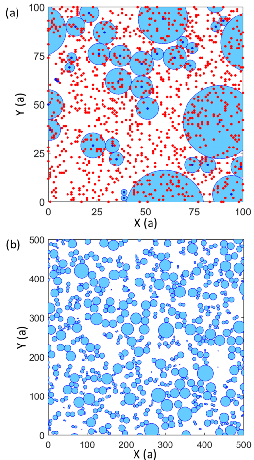
FIG. 8. (color online) Representation of the two \text{HgO}_\delta layers adjacent to a \text{CuO}_2 layer in Hg1201. (a) Red and blue dots represent randomly distributed i-O atoms with a density that corresponds to p = 0.083 (ref. 27–29 ), the doping level at which the CDW correlation length is the largest (Fig. 6). The red dots indicate unit cells with one i-O, either in the top or the bottom \text{HgO}_\delta layer. The dark blue dots indicate unit cells with two i-O, one in each of the two \text{HgO}_\delta layers. In the model considered here (see also Appendix C), CDW patches (light blue circles) nucleate in these relatively rare unit cells and extend to the closest doubly-occupied site. This results in a CDW correlation length of \xi/a \approx 7.7 , in good agreement with the experimental value \xi/a = 8.0(7) at this doping level. With increasing doping, the calculated correlation length decreases and follows the experimental values, as shown in Fig. 6(b). Displayed area: (100 a)^2 . (b) Same as in (a), but on a larger scale (displayed area: (500 a)^2 ) for better visualization of the CDW patch distribution.
