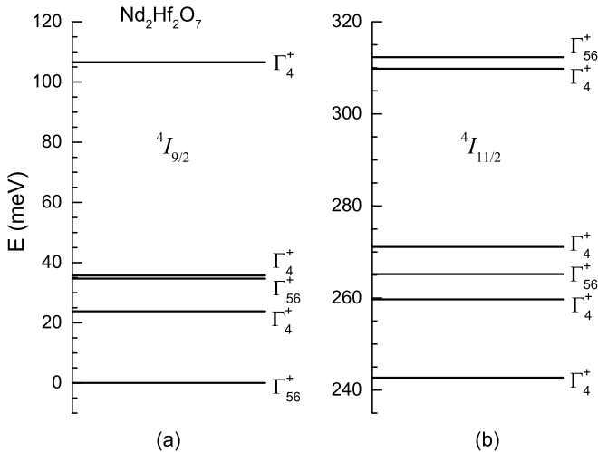
FIG. 8. (Color online) Crystal field energy schemes for (a) the ground-state multiplet {}^4I_{9/2} and (b) the first excited multiplet {}^4I_{11/2} corresponding to the crystal field parameters obtained from the analysis of INS data. \Gamma shows the irreducible representation that the corresponding CEF state transforms as.
