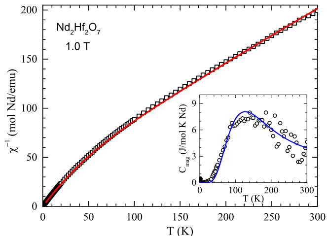
FIG. 9. (Color online) Inverse magnetic susceptibility \chi^{-1} versus temperature T of polycrystalline \text{Nd}_2\text{Hf}_2\text{O}_7 measured in a field of 1.0 T. The red solid line is the inverse crystal field susceptibility \chi_{\text{CEF}}^{-1}(T) corresponding to the crystal field parameters obtained from the analysis of INS data. Inset: Magnetic contribution to heat capacity C_{\text{mag}}(T) [22]. The blue solid curve is the heat capacity calculated from the crystal field C_{\text{CEF}}(T) .
