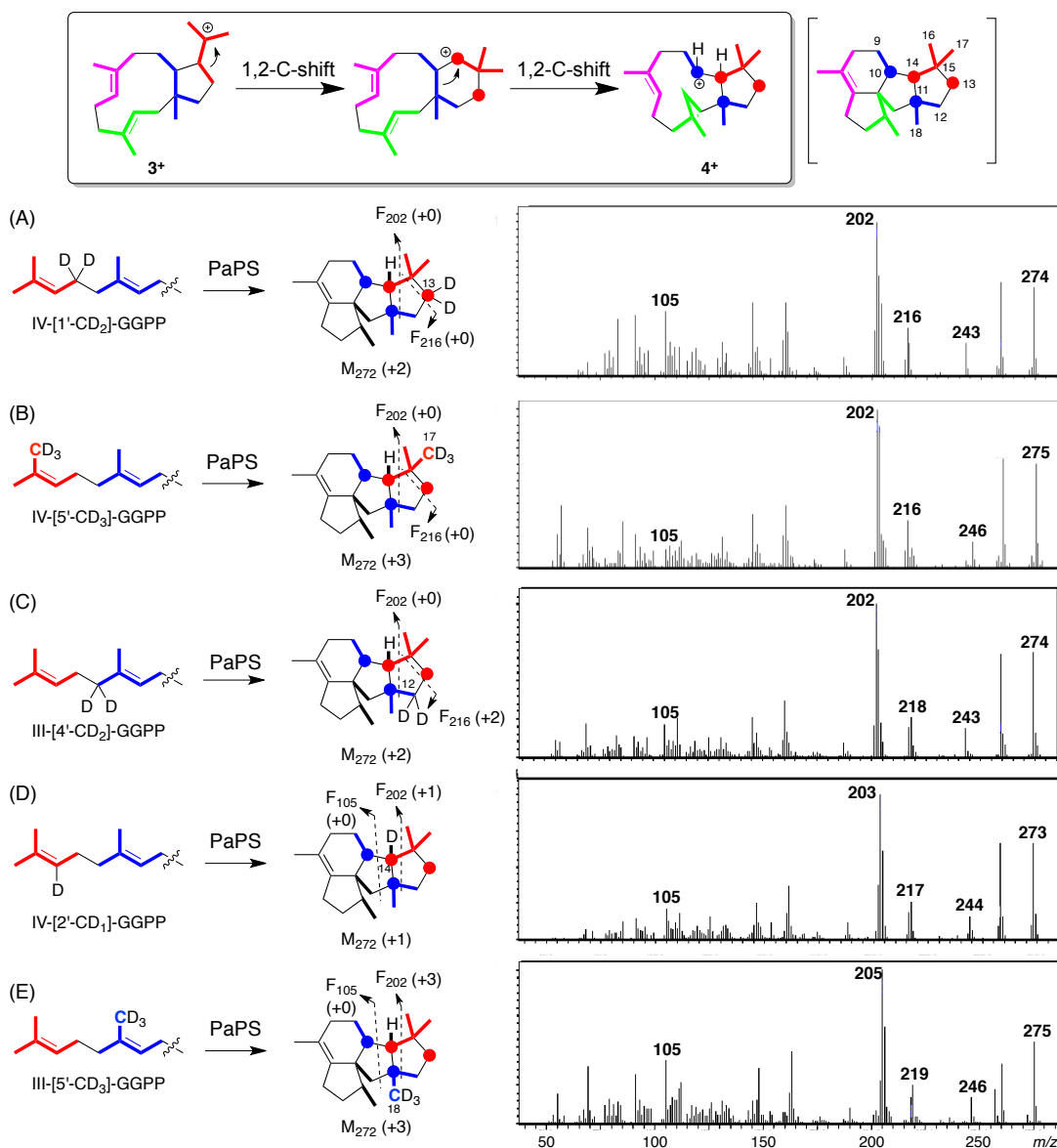
Figure 2. MS spectra of deuterium labeled 1 . The observed mass shifts are shown in the parenthesis.
