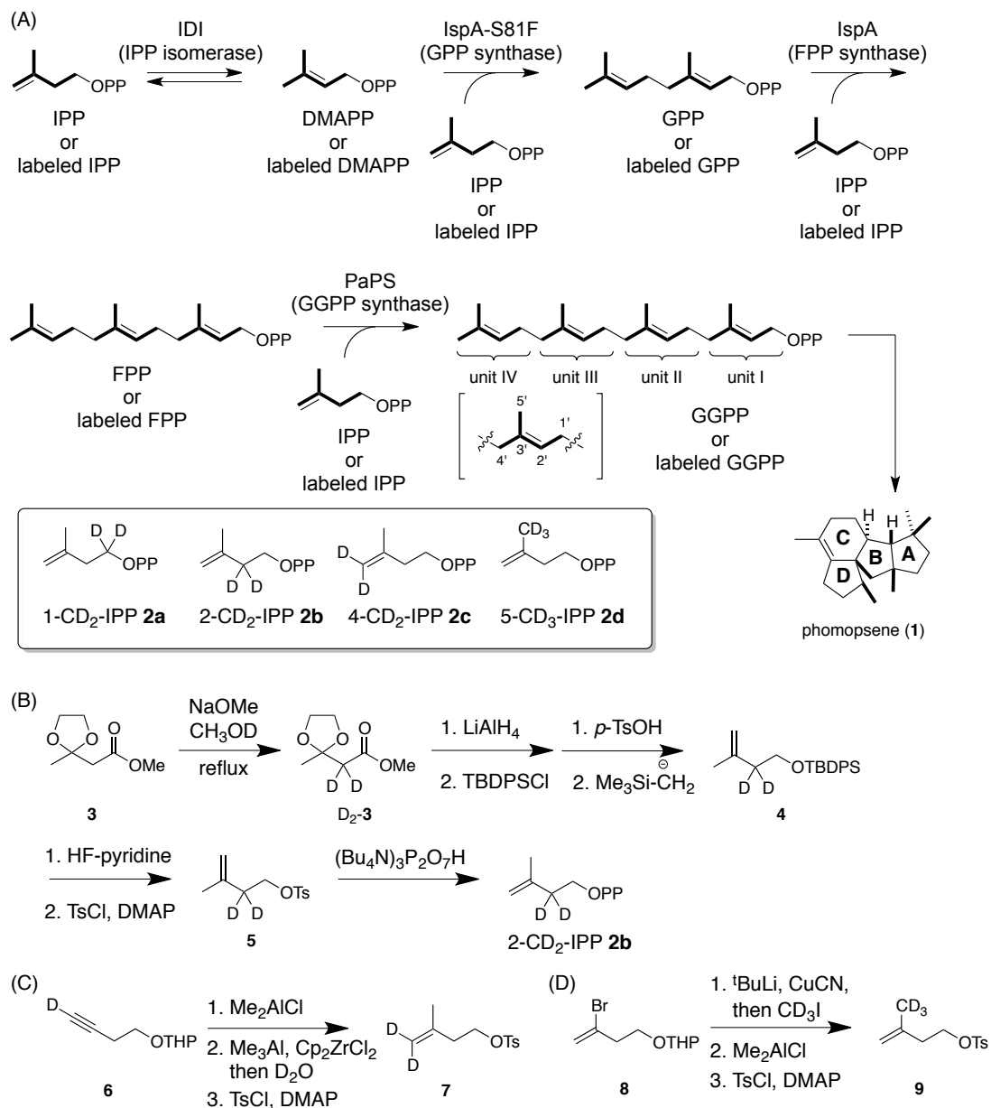
Scheme 1. (A) Outline of the chemoenzymatic synthesis of deuterium labeled 1 . Synthetic schemes of (B) 2-CD 2 -IPP 2b , (C) 4-CD 2 -IPP 2c , and (D) 5-CD 3 -IPP 2d .
