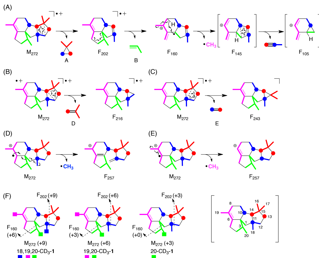
Figure 1. (A)-(E) Fragmentation sequences of 1 . (F) Fragmentations observed in 18, 19, 20- \text{CD}_3 - 1 , 19, 20- \text{CD}_3 - 1 , and 20- \text{CD}_3 - 1 .
