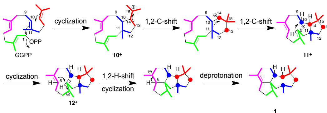
Scheme 2. Proposed cyclization mechanism of PaPS.
