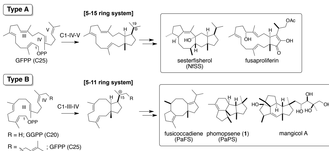
Figure 3. Classification of di/sesterterpenes based on the initial cyclization mode.
