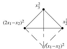
Fig. 15. Perfect cone decomposition of an FS_{2+0} + FS_1 monodromy cone.
