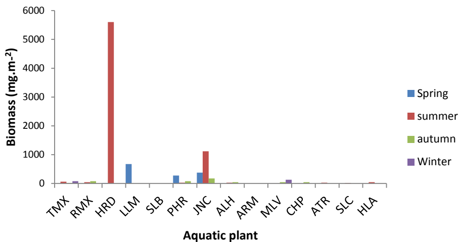
Fig 4. Change in biomass of different aquatic plants species at station 3 in different seasons (TMX - Tamarix , RMX - Rumex , ALH - Alhagi , PHR - Phragmites , JNC - Juncus , HRD - Hordeum , LLM - Lolium , SNC - Sonchus , ATR - Atriplex , INL - Inula , PLG - Polygonum , CHP - Chenopodium , MLV - Malva )
