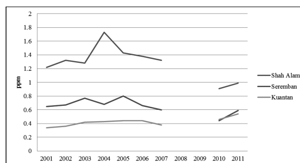
FIGURE 1. Carbon monoxide concentration in Shah Alam, Seremban and Kuantan 8 hour average daily (ppm)
