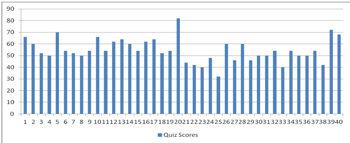
Figure 4 Data distribution of Quiz scores
