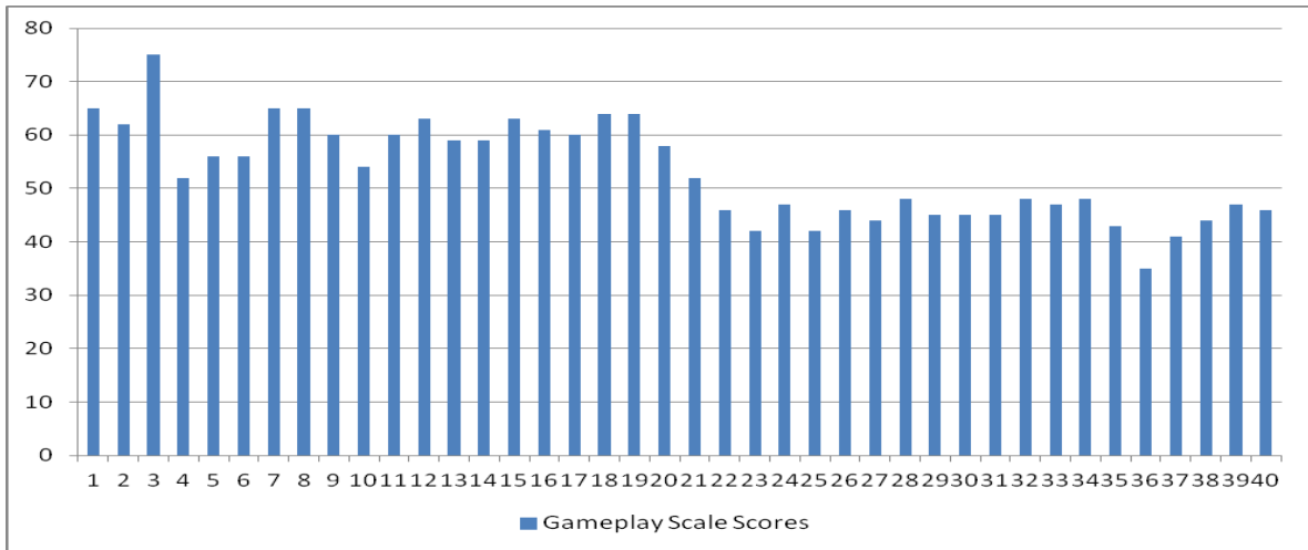
Figure 3 Data distribution of Gameplay scale score.
