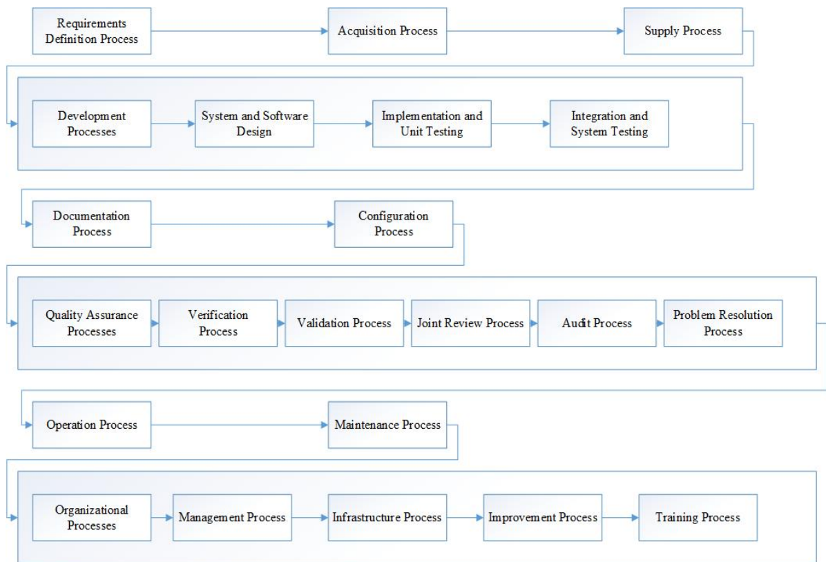
Figure 2 the diagram of selected ISO/IEC 12207: 1995 processes and their occurrence sequence during game play [29]
