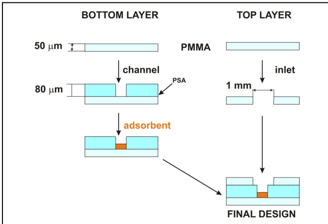
Figure 2. Schematic representation of the micro-chip fabrication;
