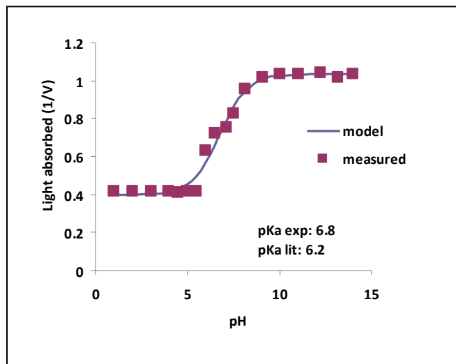
Figure 4. Calibration curve showing pH vs. light absorbed of bromocresol purple from the micro-fluidic device taken at each pH.
