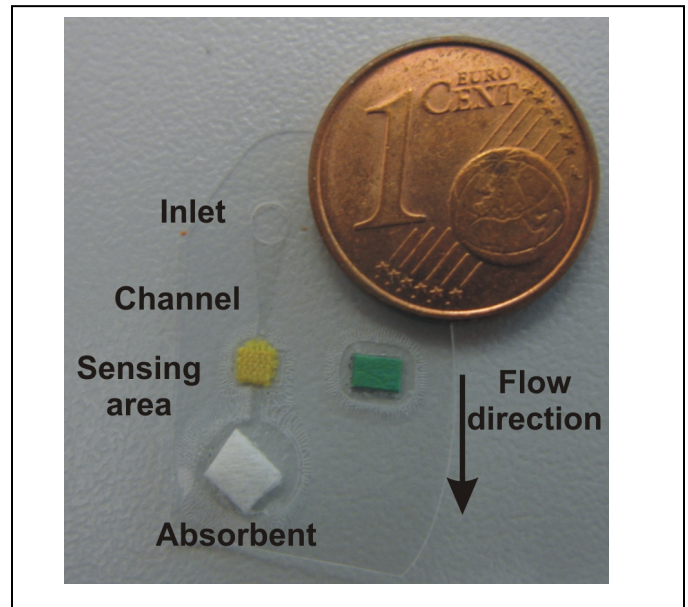
Figure 3. Picture of the micro-chip. The yellow spot is the sensing area and the green spot is the reference colour point.
