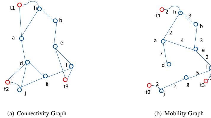
Fig. 1. Example connectivity graph and mobility graph where t_1 , t_2 and t_3 are terminals.
