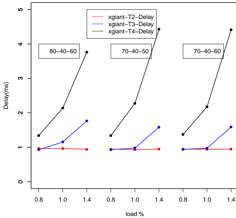
(a) Mean-delay
