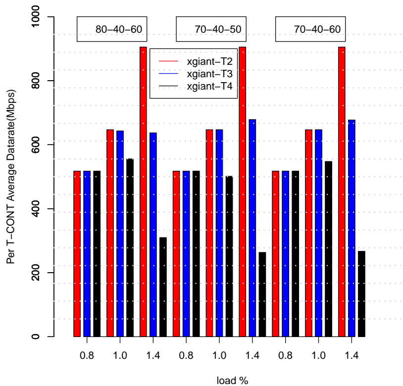
(b) Datarate
