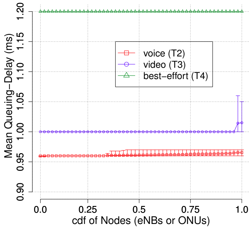
(a) XGIANT-D
