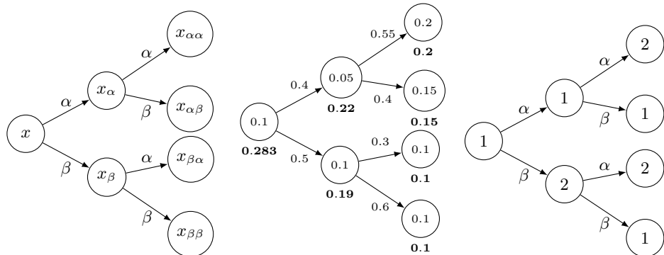
(a) Decision tree of \mathbf{A}_H . Each edge is labeled by an oracle output, and each node is labeled by an oracle input.
