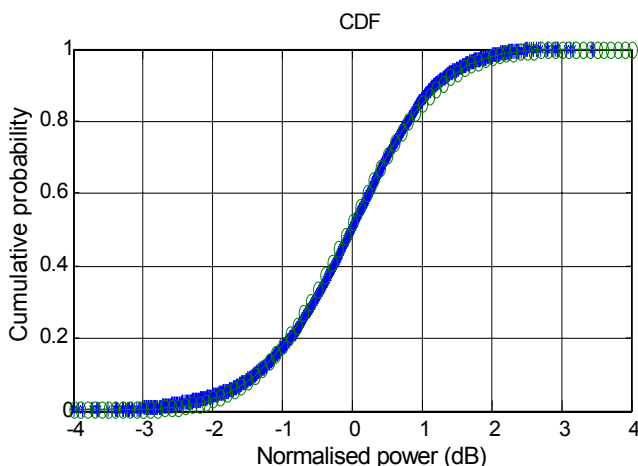
Figure 2 Cumulative distribution function of path amplitudes ('+') compared to log-normal distribution ('o') with standard deviation 1.03 dB, both in dB.
