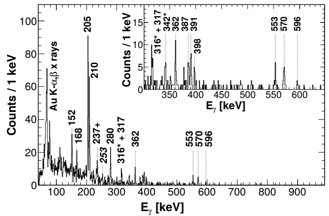
FIG. 7. Gamma rays in coincidence with \alpha decays in the region of 5944–6035 keV. The inset shows an expanded part of the spectrum for the energy region of 300–650 keV. The transition marked with the plus sign originates from the \alpha decay of ^{176}\text{Au} , transitions marked by asterisks are unassigned. Remaining \gamma -ray peaks are assigned as coincident to 5977- or 5995-keV \alpha decays of ^{180}\text{Tl} . The label in italics denotes tentative assignment.
