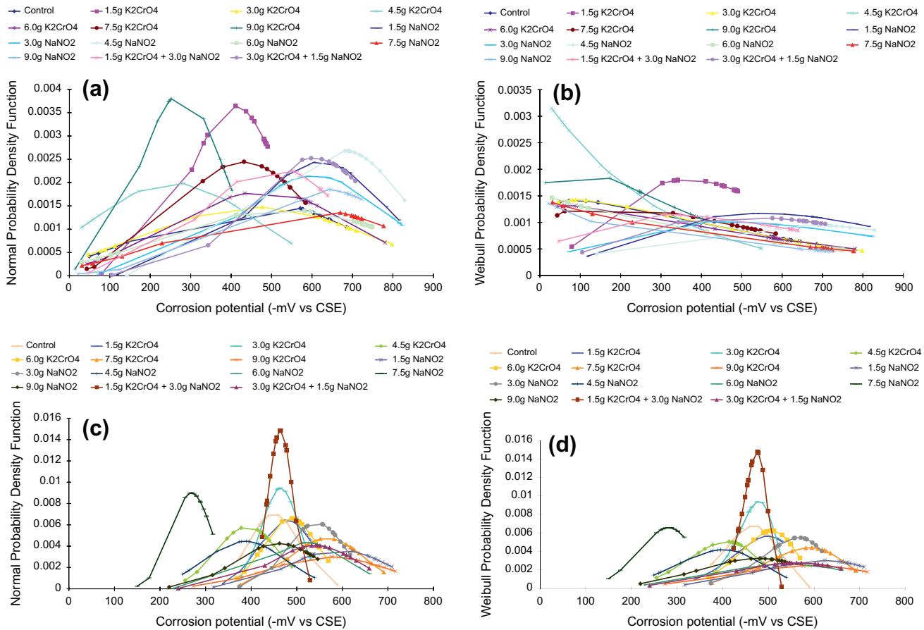
Fig. 3. Probability density function (PDF) plots for steel-reinforced concrete samples (a) Normal PDF for H 2 SO 4 -immersed samples; (b) Weibull PDF for H 2 SO 4 -immersed samples; (c) Normal PDF for NaCl-immersed samples; (d) Weibull PDF for NaCl-immersed samples.
