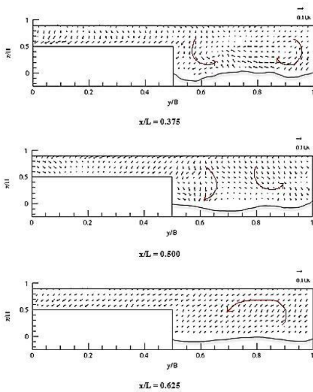
Figure 9 Distribution of secondary current along compound straight channel for deep overbank flow
