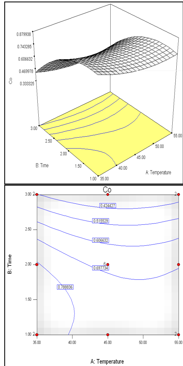
Figure 5 Surface and contour plot for cobalt content
