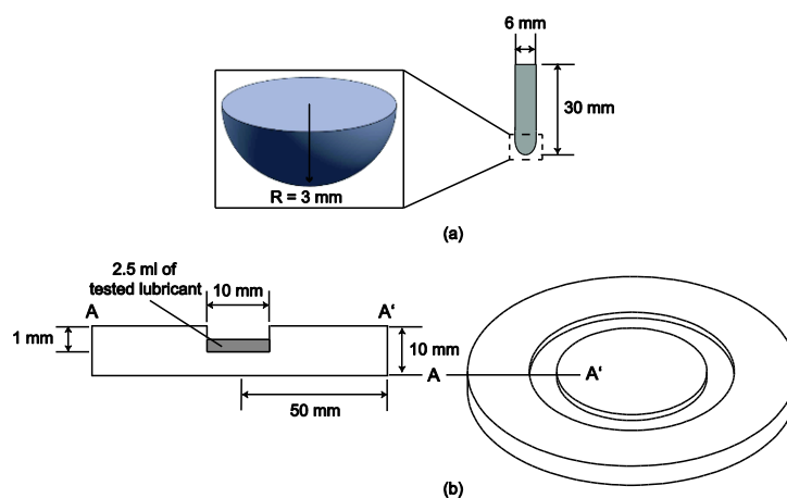
Figure 1 Geometry of the (a) pin and (b) disk
