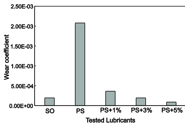
Figure 3 Wear coefficient of the pin specimen
