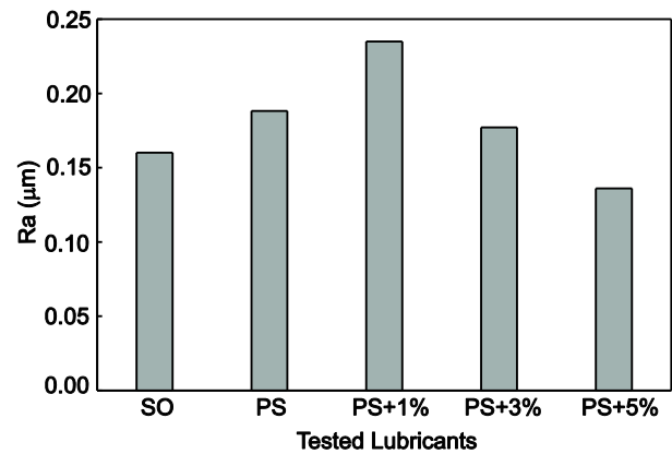
Figure 4 Arithmetic mean deviation of the surface roughness ( R_a ) of the pin specimen
