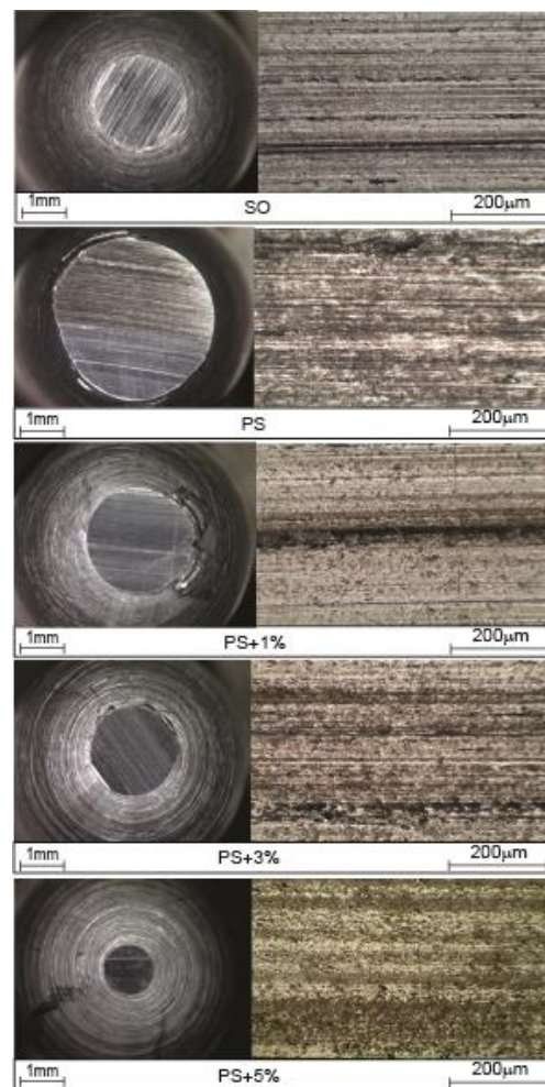
Figure 5 Physical appearance of the pin's worn surface
