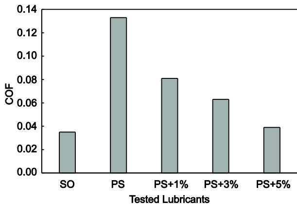
Figure 2 Coefficient of friction values at sliding speed 1.5 m/s and 9.8 N normal load
