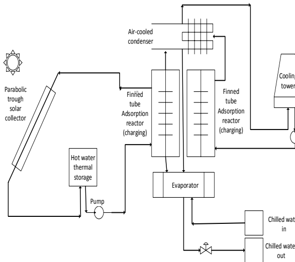
Figure 3 Adsorption chillers with hot water thermal storage
