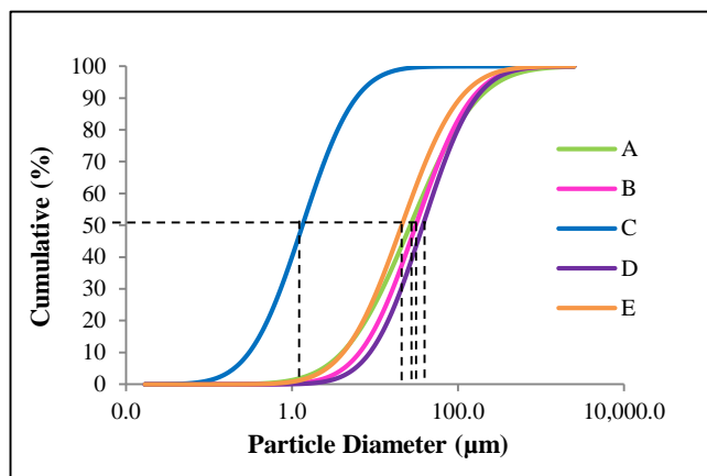
Figure 1 Cumulative particulate size distribution of fly ash from different mill
