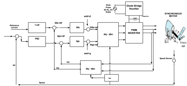
Figure 4 Vector Control Structure of the Synchronous Motor Drive
