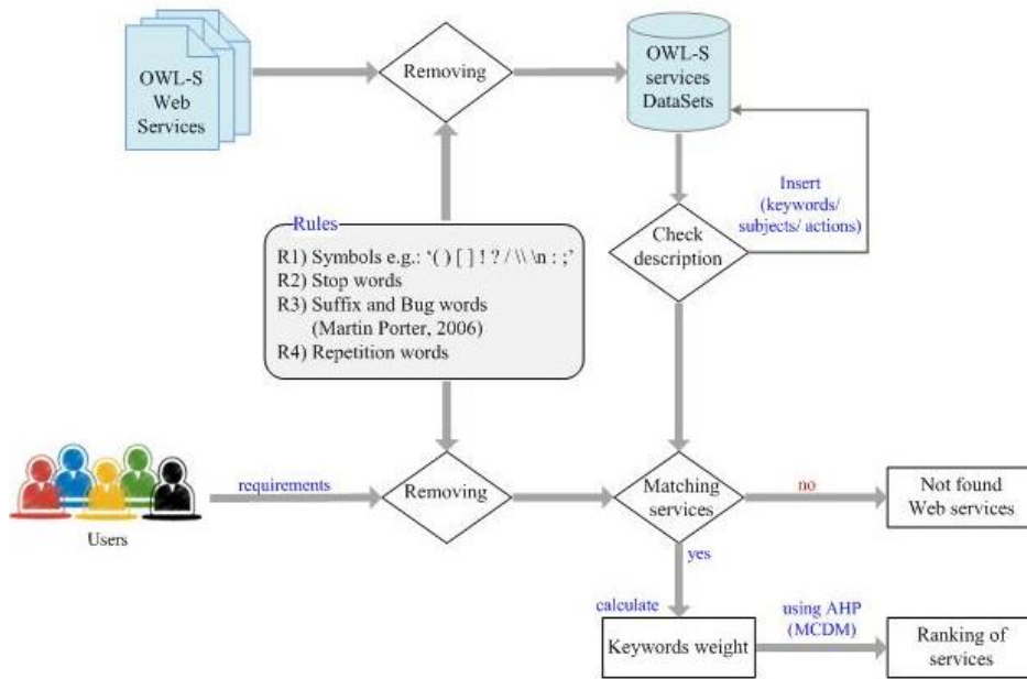
Fig. 6: Matching and ranking OWL-S service Framework
