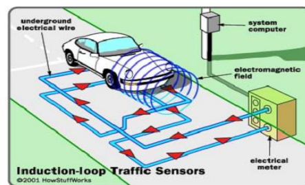
Figure 5 An inductive-loop detection system [49].
