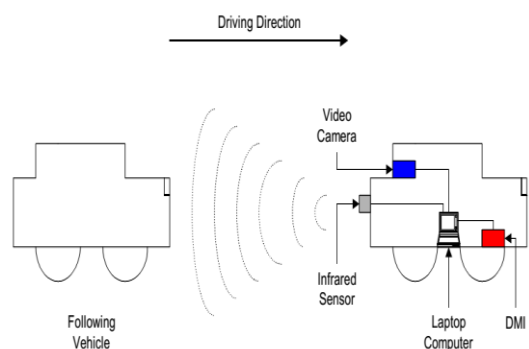
Figure 9 Example of car-following data collection apparatus [23]
