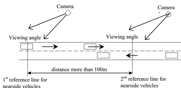
Figure 4 Arrangement of cameras for video recording process at roadside position [7].
