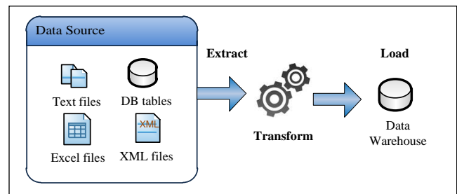
Figure 1 ETL Phases
