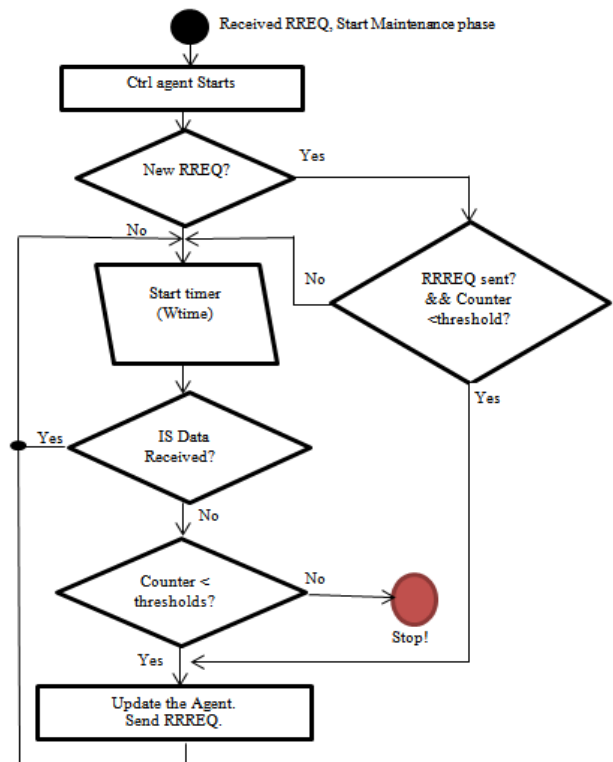
Figure 1 The path maintenance process by receiver node
