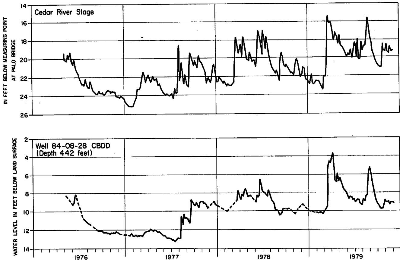
Figure 6. Stage of the Cedar River near Palo and water levels in a nearby test well completed in the Silurian aquifer (1976-1979)
