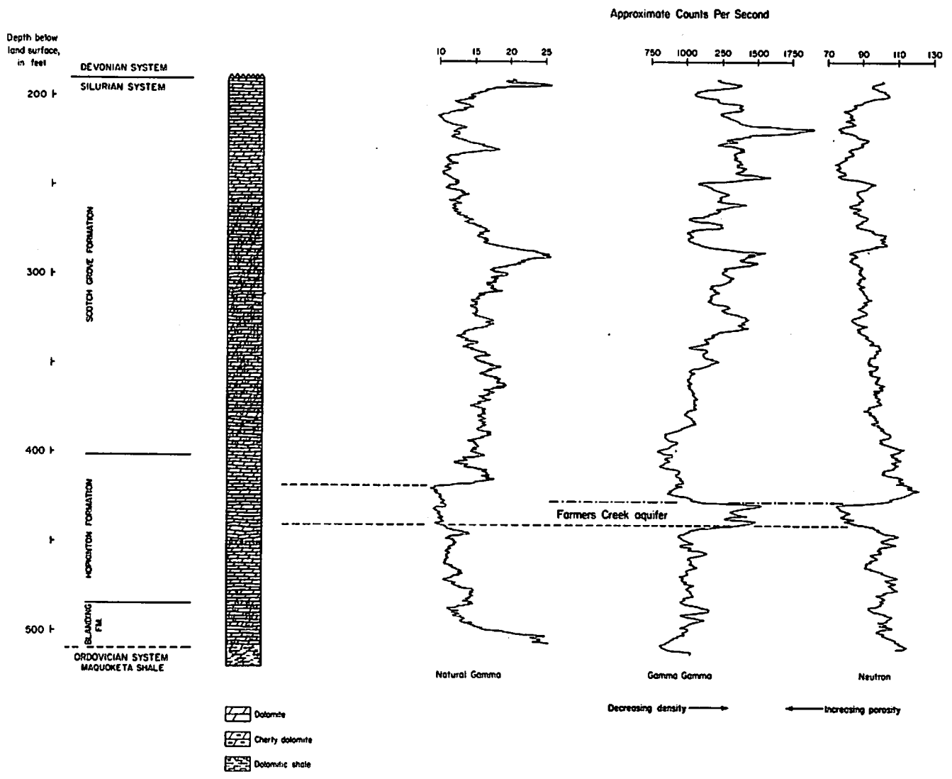
Figure 3. Lithologic log and borehole-geophysical radiation logs of a test well (84-07-16DBBB) in central Linn County.
