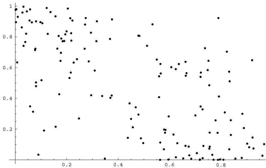
Bivariate Normality Testing with n = 15 , c = (1,1) and \text{tr}(\text{SIGMA}^{-1}S) ; data = BVGamma
