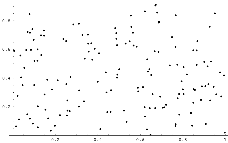
Bivariate Normality Test using n = 10 , c = (1,1) , and \text{tr}(\text{SIGMA}^{-1}S) ; data = BVN(0,I)
