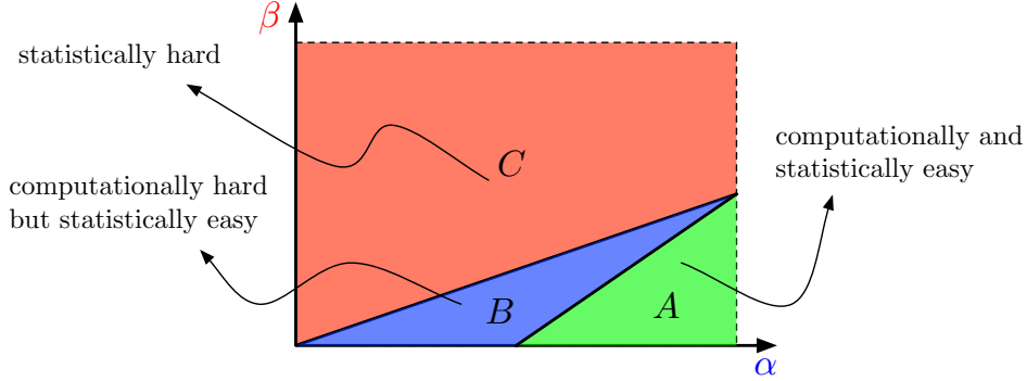
FIG 1. Phase diagram for submatrix localization. Red region (C): statistically impossible, where even without computational budget, the problem is hard. Blue region (B): statistically possible but computationally expensive (under the hidden clique hypothesis), where the problem is hard to all polynomial time algorithm but easy with exponential time algorithm. Green region (A): statistically possible and computationally easy, where a fast polynomial time algorithm will solve the problem.
