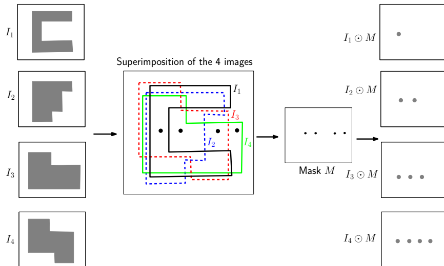
Figure 3: Unique image-indexing by geometric-set discrimination.
