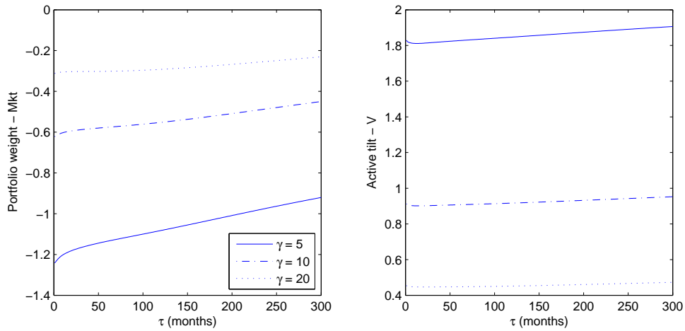
Figure 5: Stock market allocation and active value tilt implied by the optimal equity portfolio. This figure decomposes the optimal allocation to value and growth stocks (Figure 4, Panel A) into an equivalent allocation to the market portfolio and an active value tilt. The allocations are computed for investors with \gamma = \{5, 10, 20\} who can invest in cash, bonds, and the growth and value portfolios.
