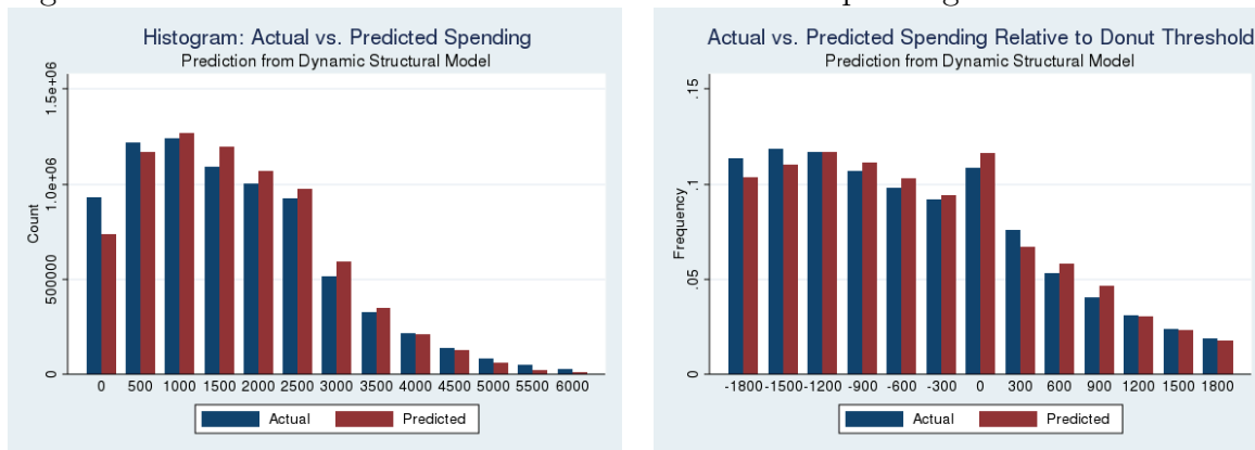
Figure 3: Distribution of Actual and Predicted Year 2 Spending – Outliers Excluded
