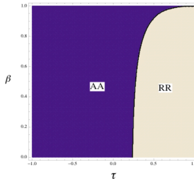
Figure A2: Channel structure when the manufacturer is the price leader in the RA configuration.
