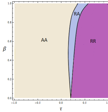
Figure 8: Channel structure when the manufacturer sells through a retailer and the prices on the traditional channel are endogenously determined ( \bar{Q} = 4 ).
