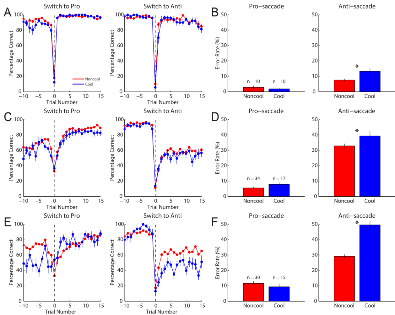
Figure 4.2. Effects of bilateral dACC deactivation on uncued switch task performance. A , Performance before and after a task switch to pro-saccades and anti-saccades during the noncool and cool periods for monkey M. Data are averaged across all experimental sessions. Trial zero is the first trial following a task switch. B , Mean error rates on the 10 trials immediately before a task switch for pro-saccades and anti-saccades during the noncool and cool periods for monkey M. Asterisks indicate a significant difference between the noncool and cool periods. C , D , and E , Same as A and B , but for monkeys C and T respectively. F , Same as B , but for monkey T.
