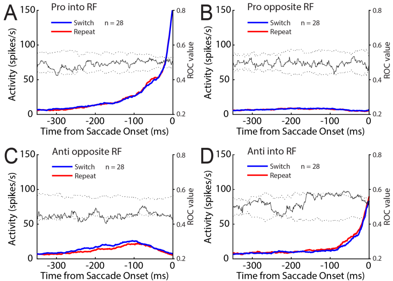
Figure 2.4. SC activity aligned to saccade onset for the gap pro- and anti-saccade task. A , Mean spike density on switch (blue) and repeat (red) trials for correct pro-saccades in which the stimulus was presented into the RF of neurons. The timecourse of average population ROC values for the comparison of switch and repeat trials is overlaid (black), with dotted lines representing the 97.5th and 2.5th percentile values obtained from a bootstrap analysis. Periods in which the solid line lies above or below the dotted lines indicate periods with significant differences ( P < 0.05 ). B , Same as A , but for correct pro-saccades in which the stimulus was presented opposite to the RF. C , D , Same as A and B , but for correct anti-saccades.
