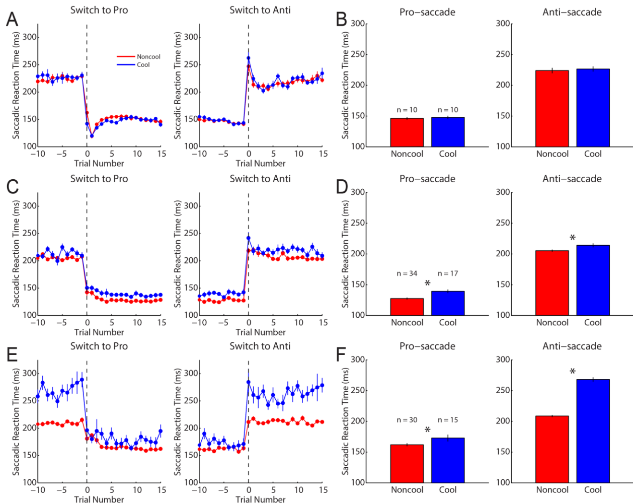
Figure 4.5. Effects of bilateral dACC deactivation on uncued switch task SRTs. A , SRTs before and after a task switch to pro-saccades and anti-saccades during the noncool and cool periods for monkey M. Data are averaged across all experimental sessions. Trial zero is the first trial following a task switch. B , Mean SRTs on the 10 trials immediately before a task switch for pro-saccades and anti-saccades during the noncool and cool periods for monkey M. Asterisks indicate a significant difference between the noncool and cool periods. C , D , and E , F , Same as A and B , but for monkeys C and T respectively.
