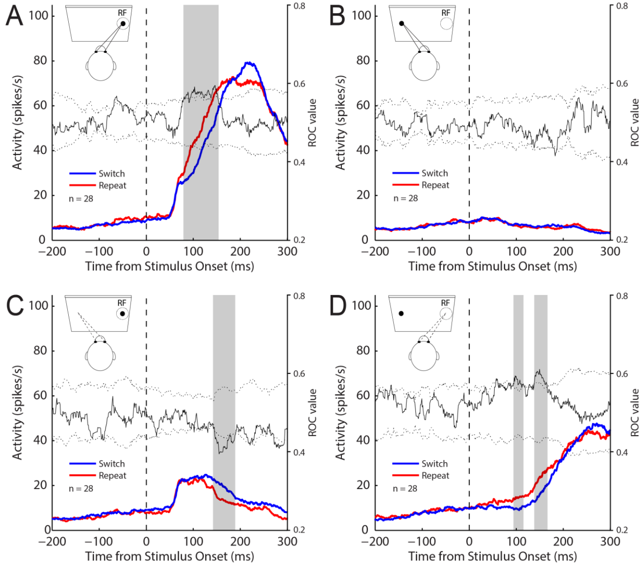
Figure 2.3. SC activity aligned to stimulus onset for the gap pro- and anti-saccade task. A , Mean spike density on switch (blue) and repeat (red) trials for correct pro-saccades in which the stimulus was presented into the RF of neurons. The timecourse of average population ROC values for the comparison of switch and repeat trials is overlaid (black), with dotted lines representing the 97.5th and 2.5th percentile values obtained from a bootstrap analysis. Periods in which the solid line lies above or below the dotted lines indicate periods with significant differences ( P < 0.05 ). The shaded region indicates a period after stimulus onset when activity for switch and repeat trials was significantly different for greater than 10 consecutive milliseconds. B , Same as A , but for correct pro-saccades in which the stimulus was presented opposite to the RF. C , D , Same as A and B , but for correct anti-saccades.
