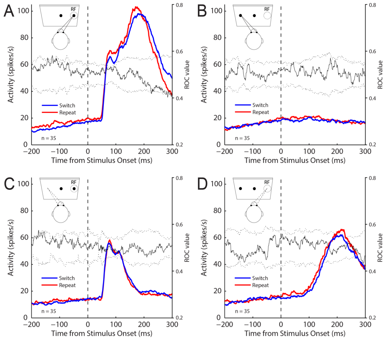
Figure 2.5. SC activity aligned to stimulus onset for the memory pro- and anti-saccade task. A , Mean spike density on switch (blue) and repeat (red) trials for correct pro-saccades in which the stimulus was presented into the RF of neurons. The timecourse of average population ROC values for the comparison of switch and repeat trials is overlaid (black), with dotted lines representing the 97.5th and 2.5th percentile values obtained from a bootstrap analysis. Periods in which the solid line lies above or below the dotted lines indicate periods with significant differences ( P < 0.05 ). B , Same as A , but for correct pro-saccades in which the stimulus was presented opposite to the RF. C , D , Same as A and B , but for correct anti-saccades.
