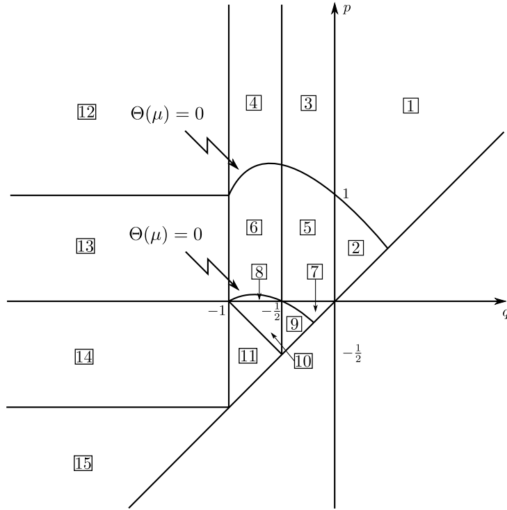
Figure 5: Sketch of the regions in the proof of Lemma 2.5.
