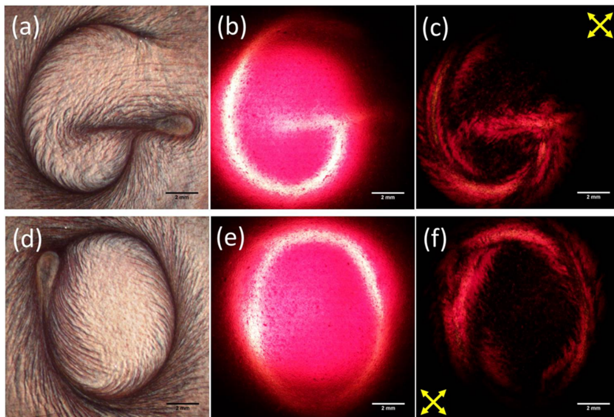
Figure 9: Images of a defined structure in a liquid crystalline e-ink of graphene oxide dispersed in water in (a,d) reflection with unpolarised light, (b,e) transmission with unpolarised light and (c,f) transmission between crossed polarisers. Reproduced from He et al , Nanoscale , 2014 52 with permission from The Royal Society of Chemistry ©2014.
