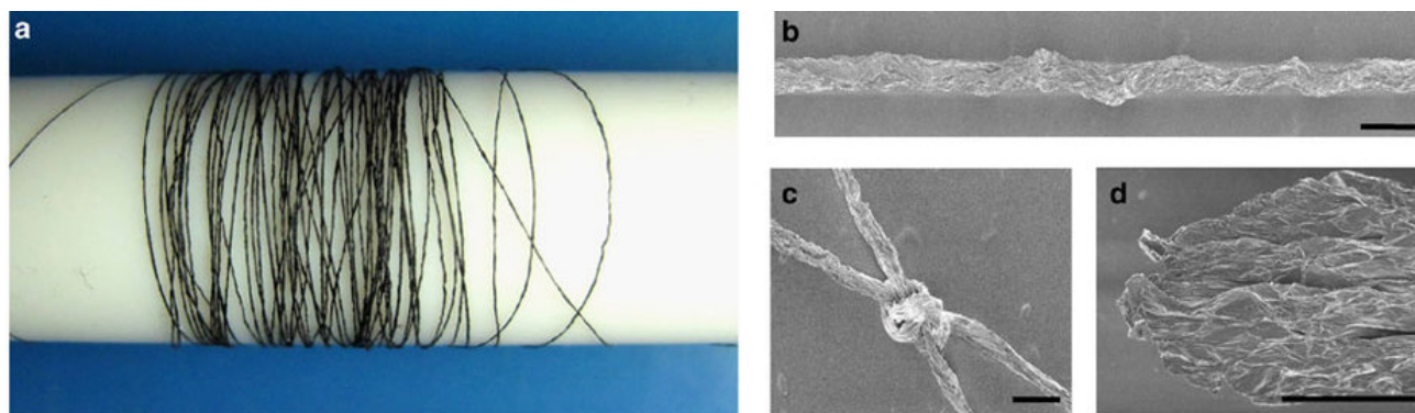
Figure 7: (a) Four-metre-long wound GO fibre. SEM images of the fibre (b), and a typical tighten knot (c). (d) The morphology of the GO fibre after tensile tests. All scale bars 50 \mu\text{m} . Reproduced with permission from Xu & Gao, Nature Communications , 2011 4 . (©2011 Nature Publishing Group).
