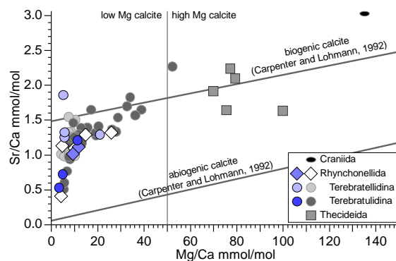
Fig. 3. Cross plot of average Sr/Ca and Mg/Ca ratios in the studied brachiopod species (blue colours) supplemented with results from Lowenstam (1961), Carpenter and Lohmann (1992, 1995), Brand et al. (2003, 2013), Lee et al. (2004), Pérez-Huerta et al. (2008) (white, grey, and black). The approximate limit of low-Mg calcite as well as proposed trend lines for abiogenic and biogenic calcite (Carpenter and Lohmann, 1992) are also indicated.
